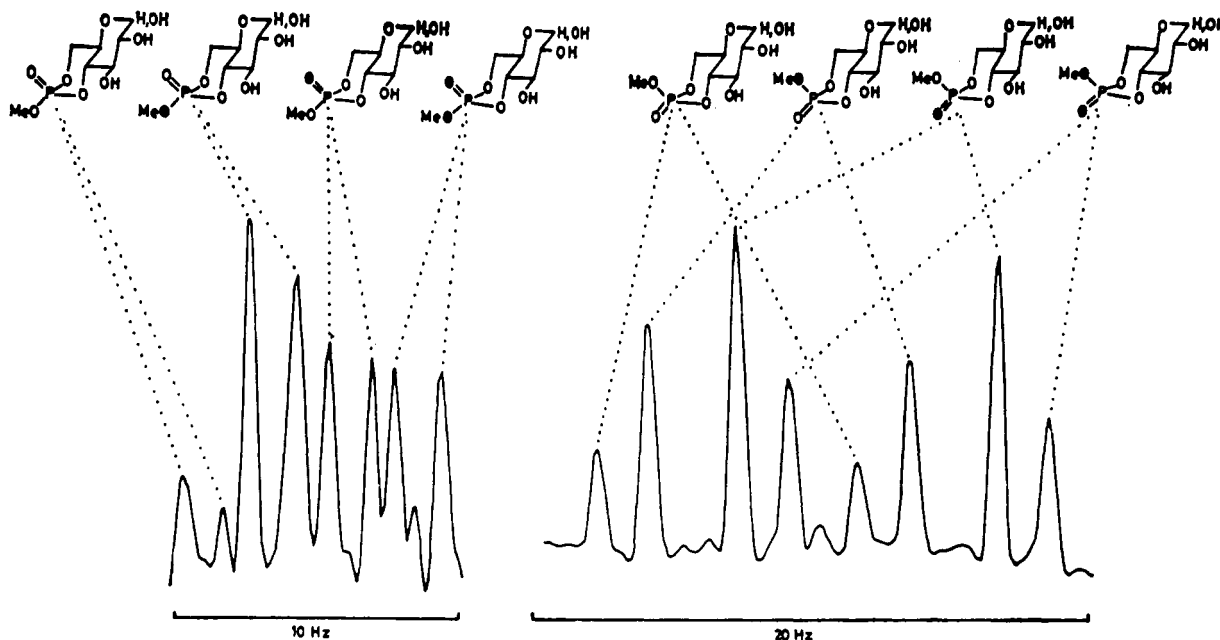
Figure 1. The ^{31}\text{P} NMR spectrum (121.5 MHz) of the axial and equatorial triesters obtained by cyclization and esterification of D-glucose 6-[(S)- ^{16}\text{O} , ^{17}\text{O} , ^{18}\text{O} ]phosphate ( \bullet = ^{18}\text{O} ).
