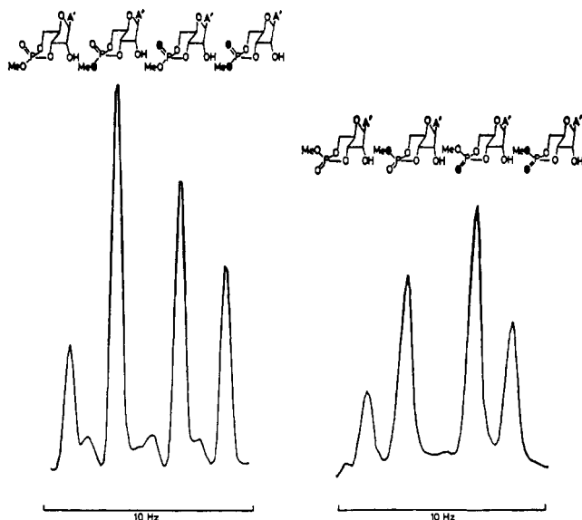
Figure 2. The ^{31}\text{P} NMR spectrum (121.5 MHz) of the axial and equatorial triesters obtained by cyclization and methylation of adenosine 5'-[(S)- ^{16}\text{O} , ^{17}\text{O} , ^{18}\text{O} ]phosphate ( \bullet = ^{18}\text{O} , A' = N-methyladenine).
